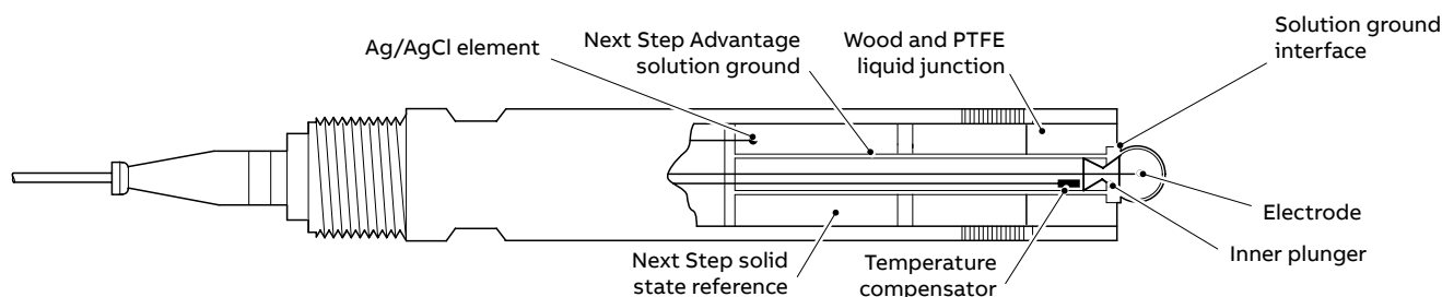
01 ABB TB(X)5 series sensor construction
